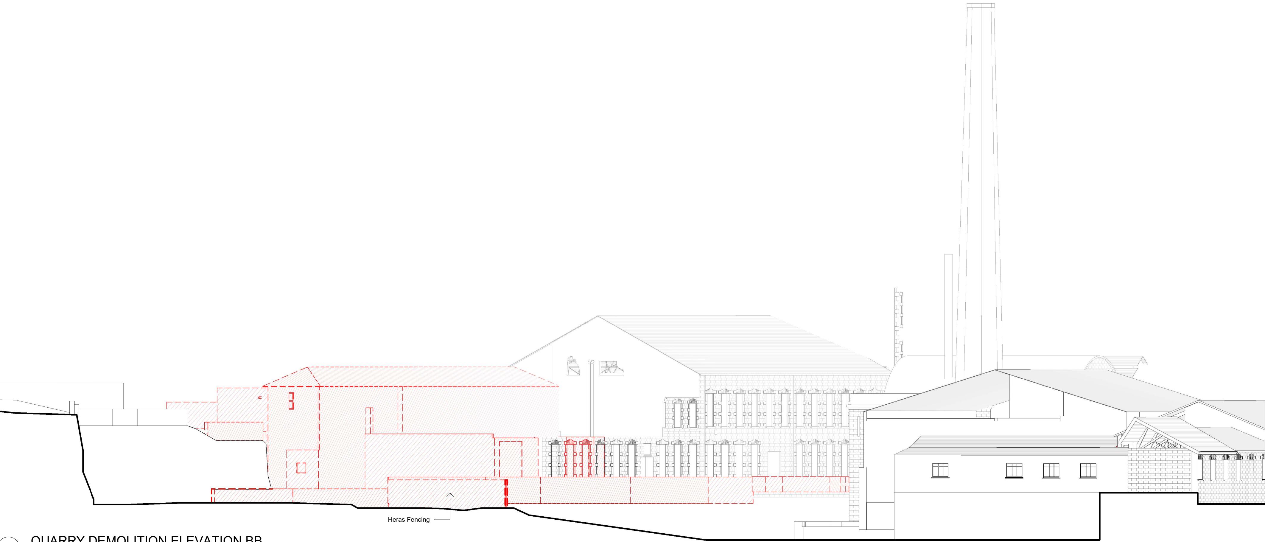
2 QUARRY DEMOLITION ELEVATION BB 1 : 200
